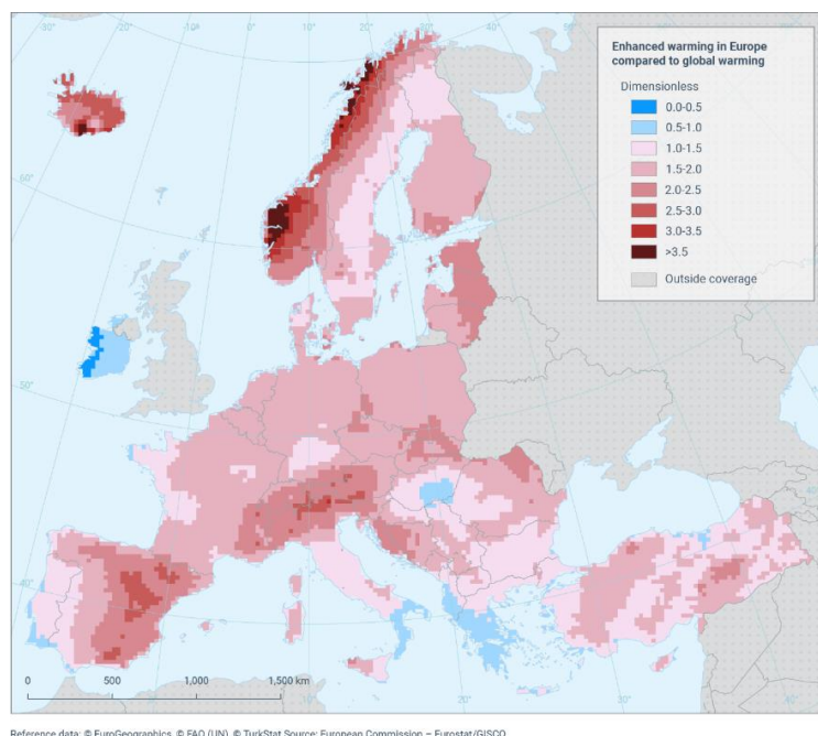
Figure 1 Enhanced warming in Europe compared to global warming. Figure 2.3 from the EUCRA report.
