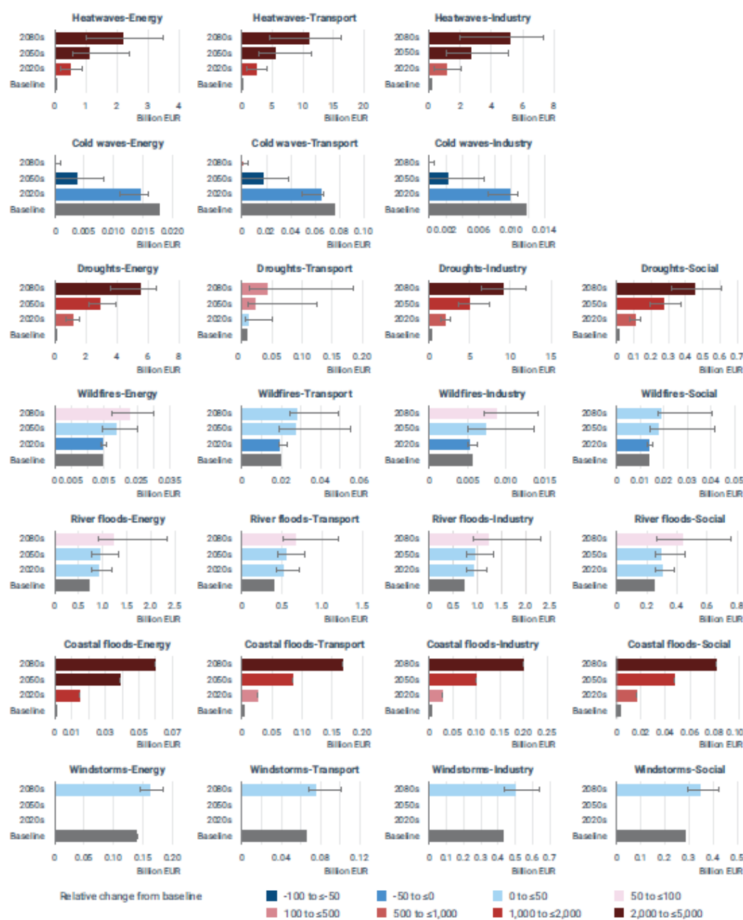
Figure 15.2 Expected annual damage to critical infrastructure assets
